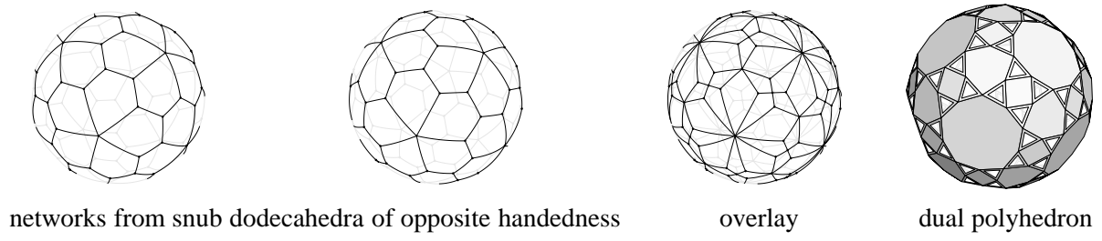
Figure 4 Another polyhedron created with the dualization technique.
