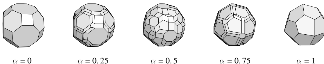
Figure 7 A linear combination (1 - \alpha)P_1 + \alpha P_2 , where P_1 is a truncated cuboctahedron and P_2 is a pentagonal icositetrahedron. The dual networks of each combination are all identical, except for the weights on each arc.
